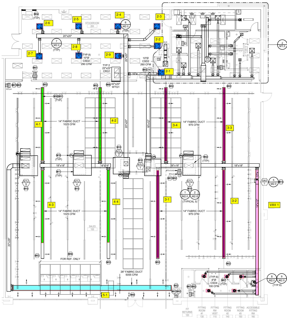
① HVAC PLAN 1/8" = 1'-0"
